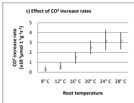
Figure 1. The distribution of water uptake rates (a), the effects of O 2 decrease rates (b) and CO 2 increase rates (c) on root temperature in root systems under 80 kPa suction. Mean values from 6 plants are plotted with 95% confidence interval.
