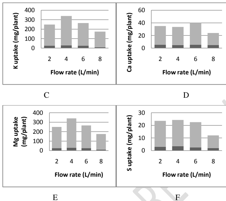
Figure 2. Plant nutrient uptake varies with flow rate. Plants absorb a) nitrogen, b) phosphorus, c) potassium, d) calcium, e) magnesium, f) sulphur. Significant differences were observed between the bars labelled with different letters ( p < 0.05 ). The data are presented as means \pm standard error ( n = 4 ).
