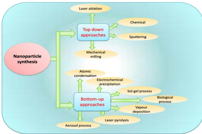
Fig no 2 :Nanoparticle synthesis
