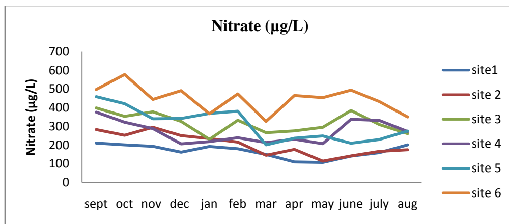
Figure 12: Monthly Variation in Nitrate-nitrogen ( \mu\text{g/L} ) at different sites in Dachigam Stream
