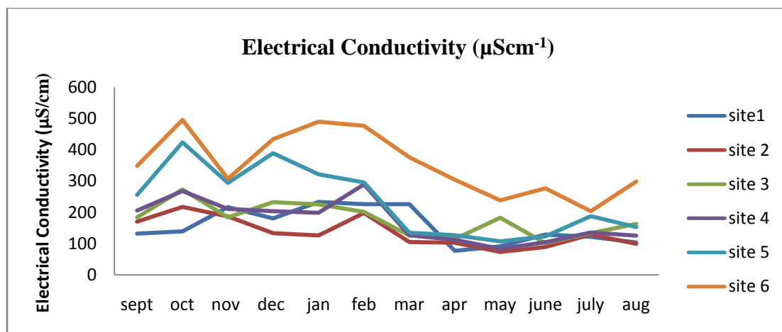
Figure 7: Monthly Variation in Electrical conductivity ( \mu\text{S}/\text{cm} ) at different sites in Dachigam Stream
