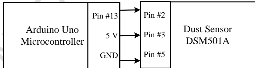
Fig.4. Connection diagram of the DSM501A with Arduino Uno [18].
