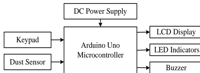
Fig. 1. Block diagram of the proposed scheme.
