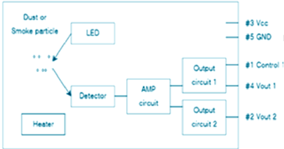
Fig.3. Block diagram of the DSM501A sensor [17].
