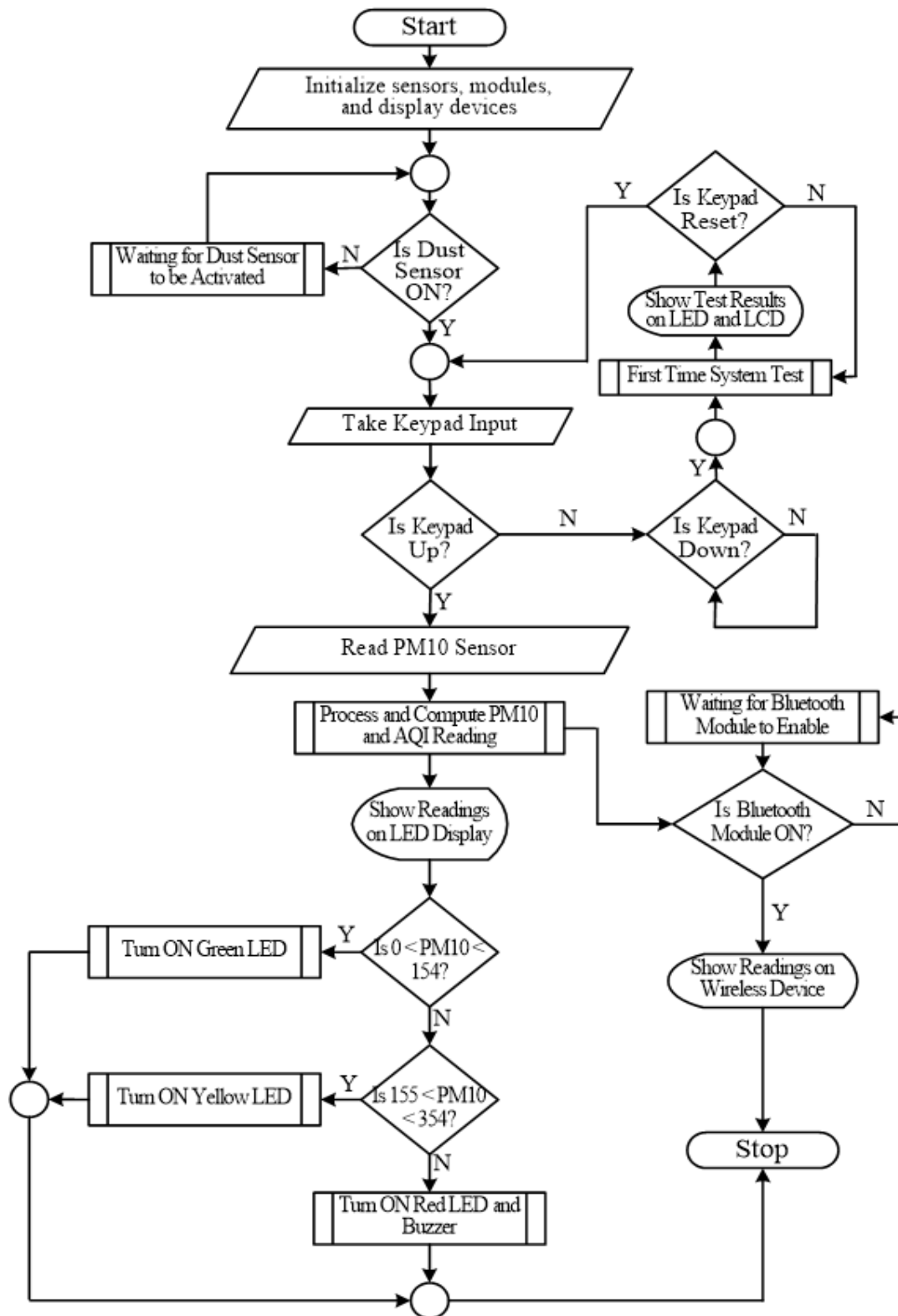
Fig.2.Flowchart of the proposed system.
