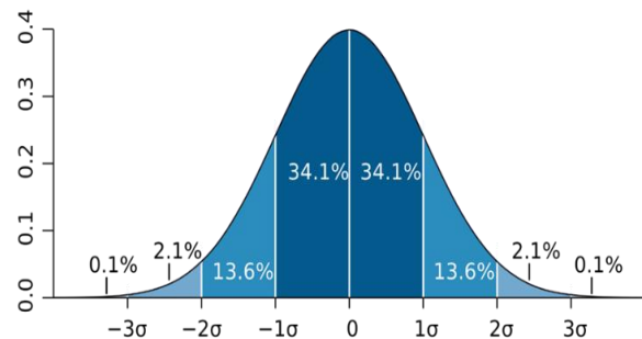
Fig 1. Bell-shaped curve [3]
