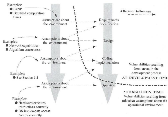
Fig. 1. Software Vulnerability Theory
