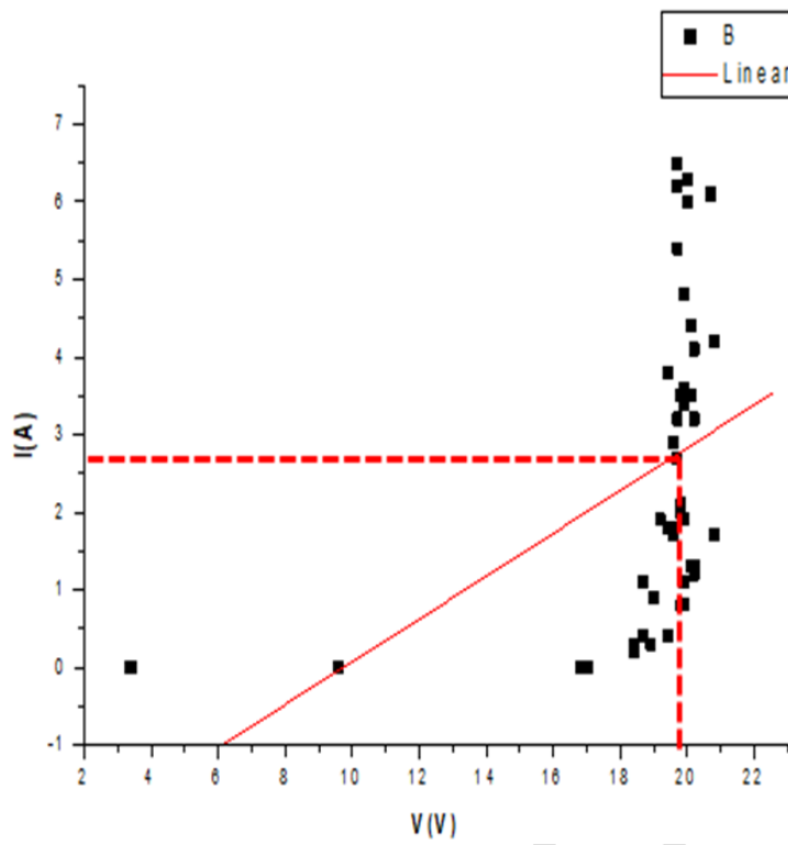
Figure 2: A Graph of Current Against Voltage of Monocrystalline for Okuku
