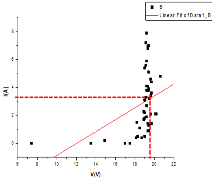
Figure 4: A Graph of Current Against Voltage of Polycrystalline for Okuku
