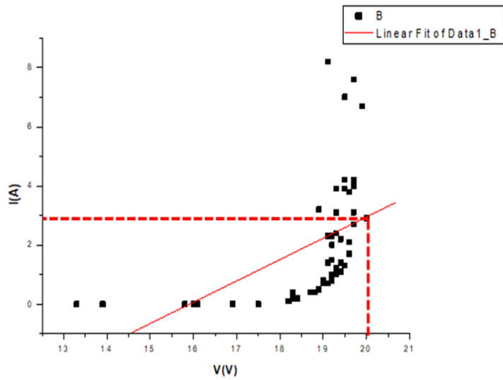
Figure 5: A Graph of Current Against Voltage of Polycrystalline for Calabar
