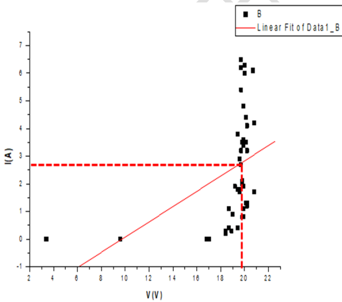
Figure 4: A Graph of Current Against Voltage of Monocrystalline for Okuku
