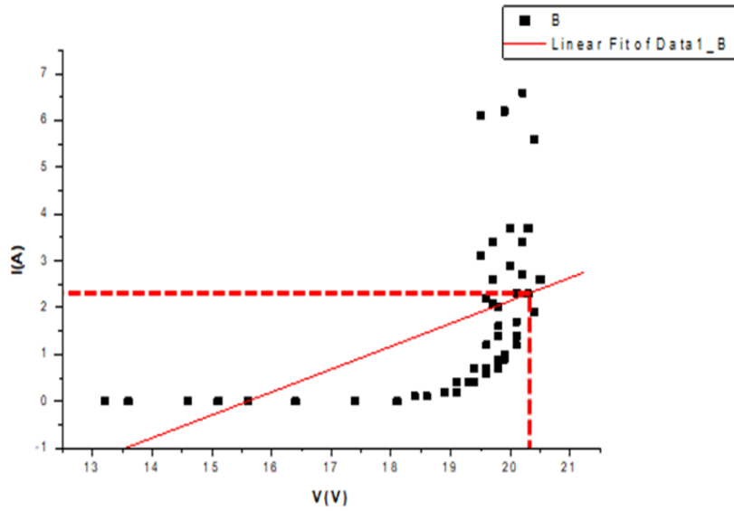
Figure 3: A Graph of Current Against Voltage of Monocrystalline for Calabar
