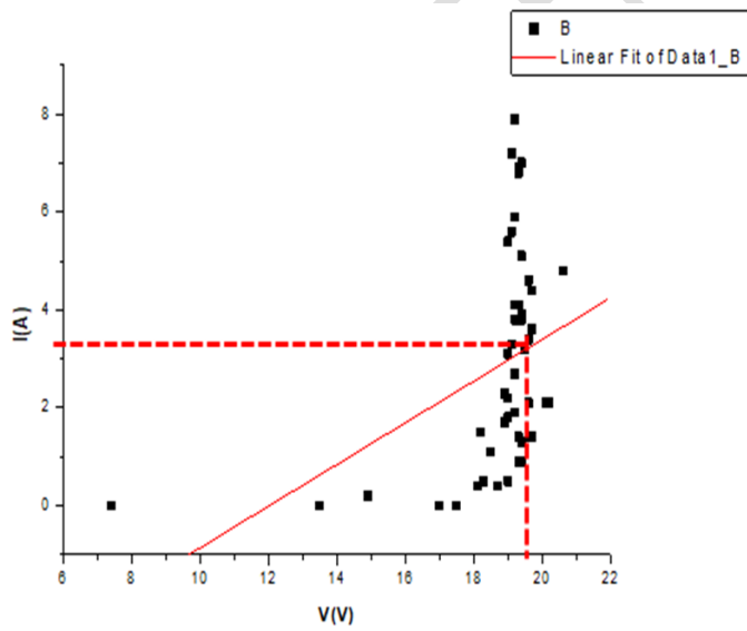
Figure 6: A Graph of Current Against Voltage of Polycrystalline for Okuku
