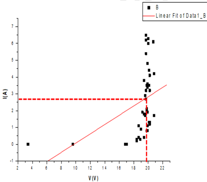
Figure 4: A Graph of Current Against Voltage of Monocrystalline for Okuku
