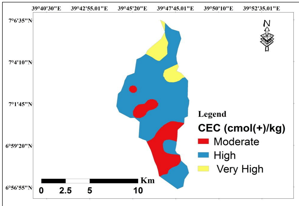
Figure 4. Soil cation exchange capacity (CEC) status map of the Danka watershed in Dinsho District.
