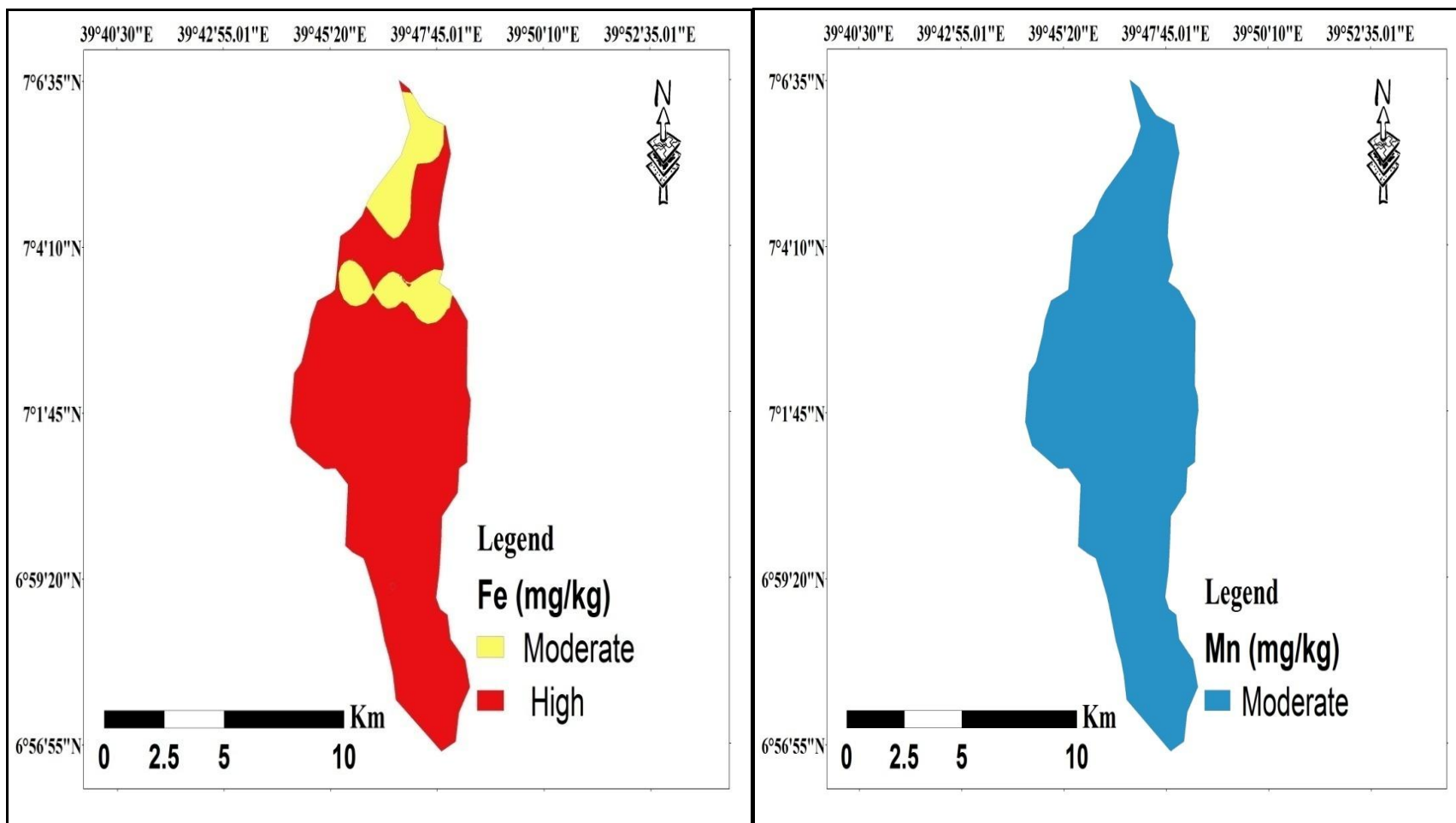
Figure 8. Soil iron (Fe) and manganese (Mn) status map of the Danka watershed in Dinsho District.
