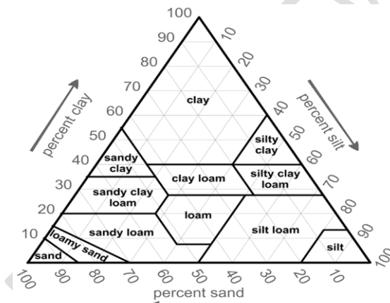
Fig 2. If the percentages of sand, silt, and clay are known, a soil textural triangle can be used to determine soil texture (source: USDA).
