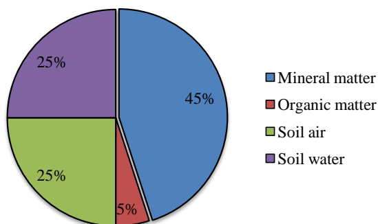
Fig1. Mineral particles, water, air, and soil are all soil components.
