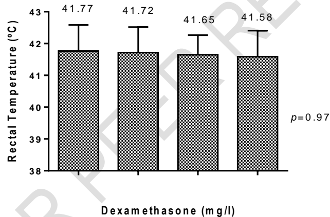
Figure 2: Rectal temperatures of broiler chickens fed betaine HCl under dexamethasone induced stress
