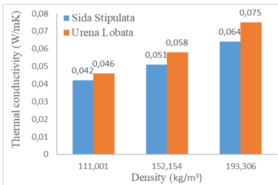
Fig. 5. Thermal conductivity as a function of density
