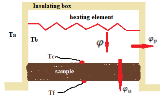
Fig. 3. Sample in thermal box
