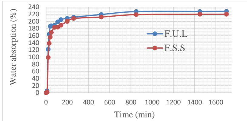
Fig. 4. Water absorption of fibers
