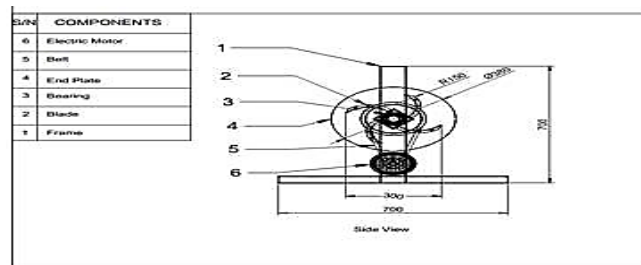
Figure 9: Orthographic diagram with side view of the turbine
