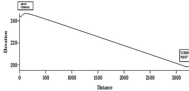
Figure 6: Evaluation of pumping head from reservoir
