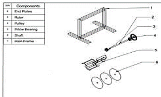
Figure 11: Exploded view of the turbine
