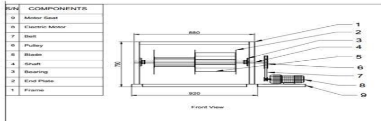
Figure 8: Orthographic diagram with front view of the turbine
