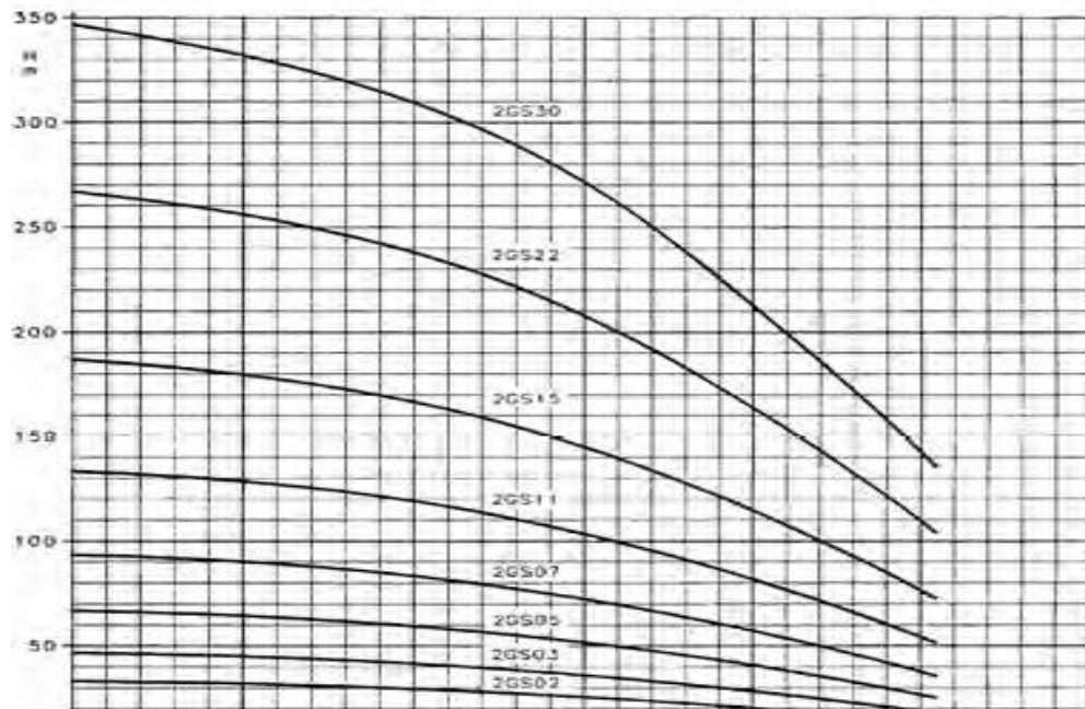
Figure 7: Lowara Xylem 2GS (2024) pump catalogue chart
