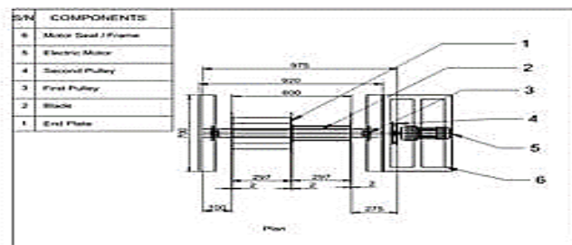
Figure 10: Plan view of the turbine
