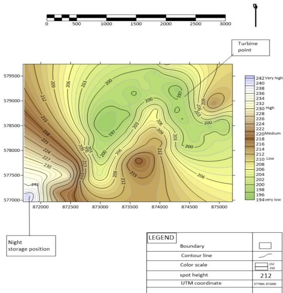
Figure 5: Contour map showing elevation of Night Storage and Turbine Point
