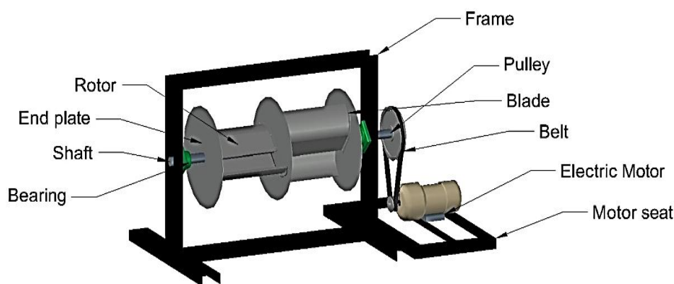
Figure 12: Isomeric view of Savonius turbine
