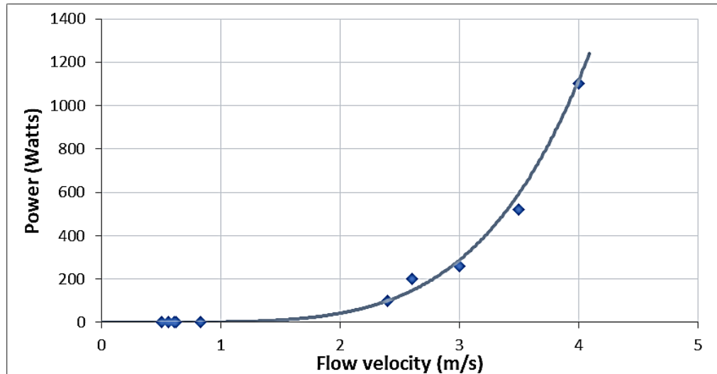
Figure 13: The Savonius hydrokinetic power curve
