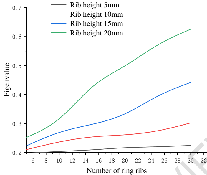
Fig10 Optimization results of large size pressure stability
