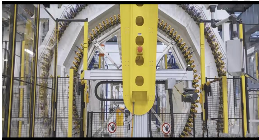
Fig3 British two-ring knitting machine
