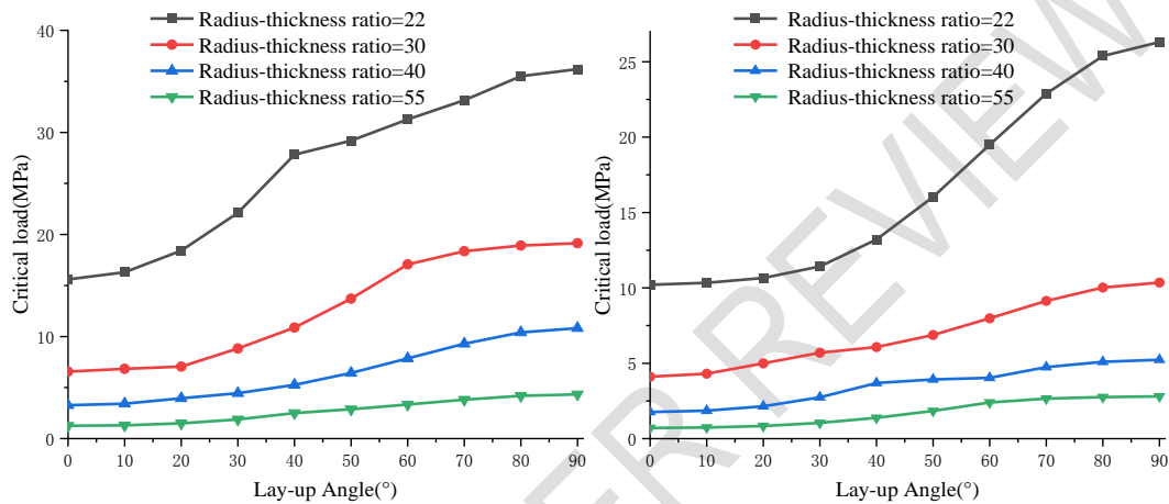
Fig7 Relation of winding Angle of cylinder with different length and critical load under different aspect ratio
