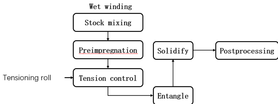
Fig5 Winding diagram
