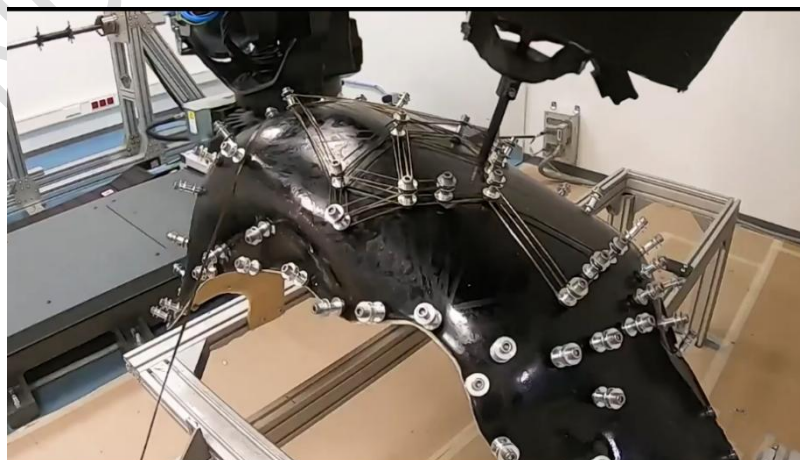
Fig8 Robot winding
