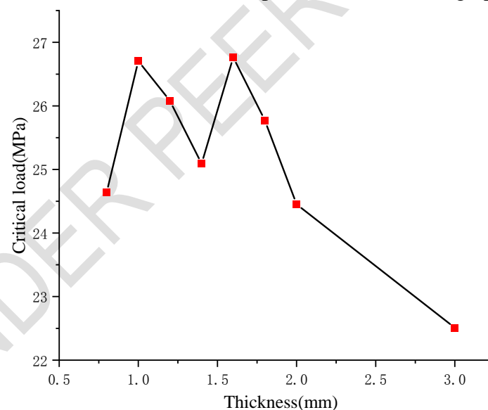
Fig12 Relationship between critical load and thickness of titanium alloy layer
