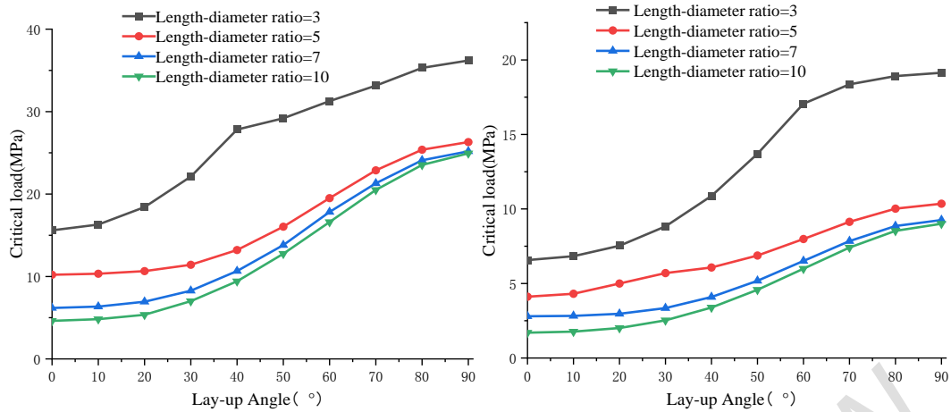
Fig10 Relation of winding Angle of cylinder with different length and critical load under different diameter thickness ratio
