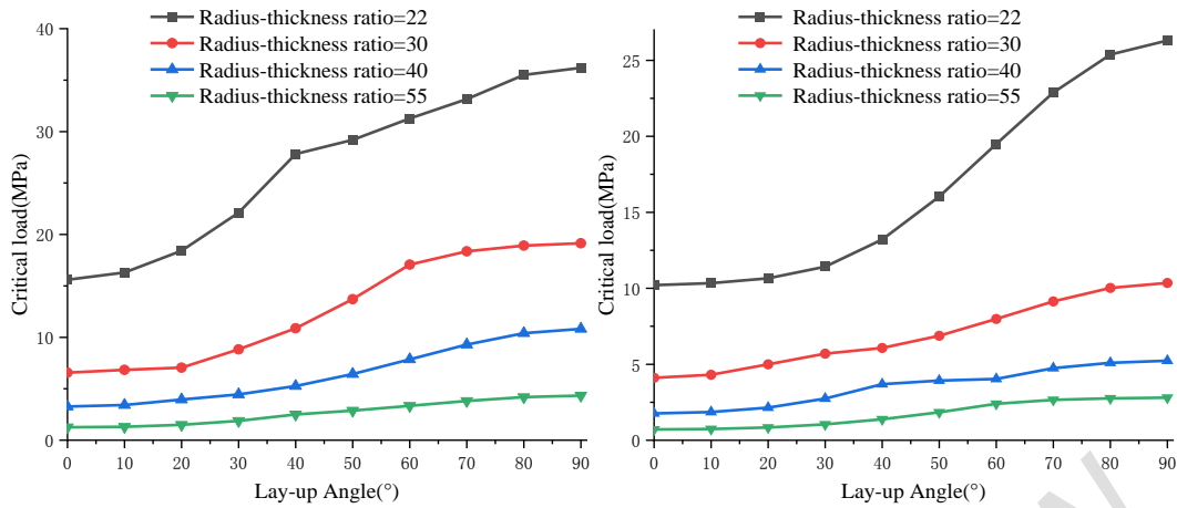
Fig.11 Relation of winding Angle of cylinder with different length and critical load under different aspect ratio
