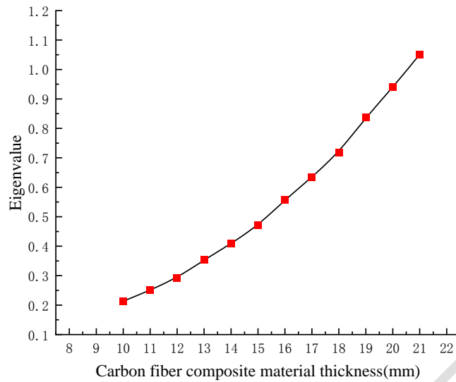
Fig13 The relationship between thickened tank body and characteristic value
