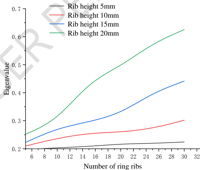
Fig14 Optimization results of large size ballast stability
