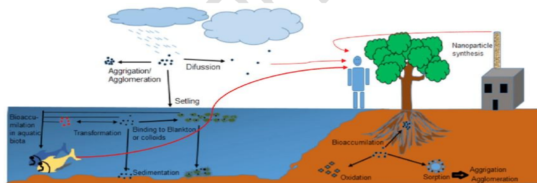
Figure 2 illustrates the potential environmental fate and behavior of nano-pesticides.
