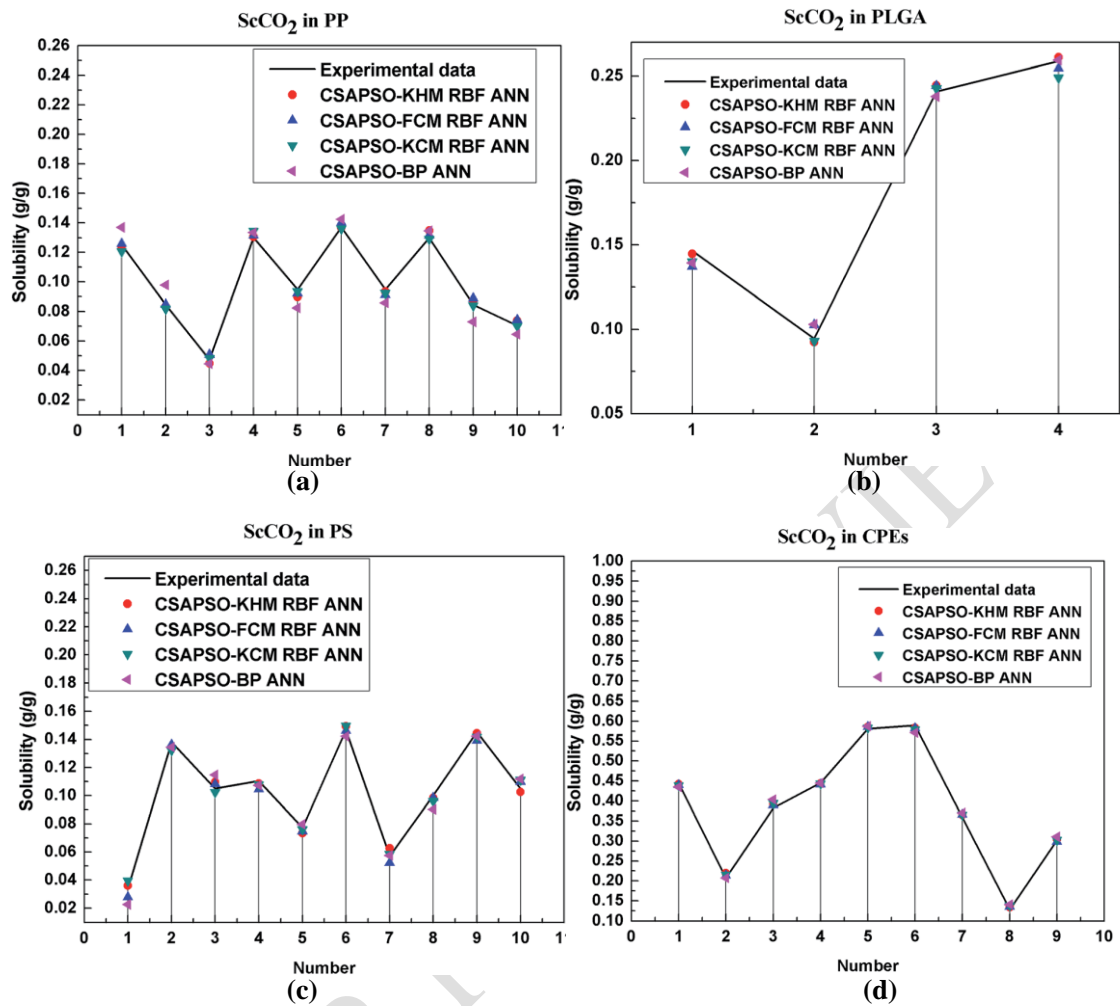
Fig. 7 Prediction of \text{ScCO}_2 in 4 polymers[37]
