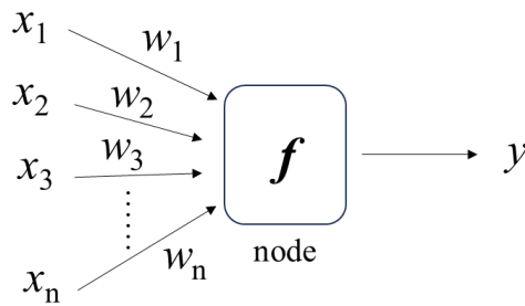
Fig. 5 The basic model of ANN
