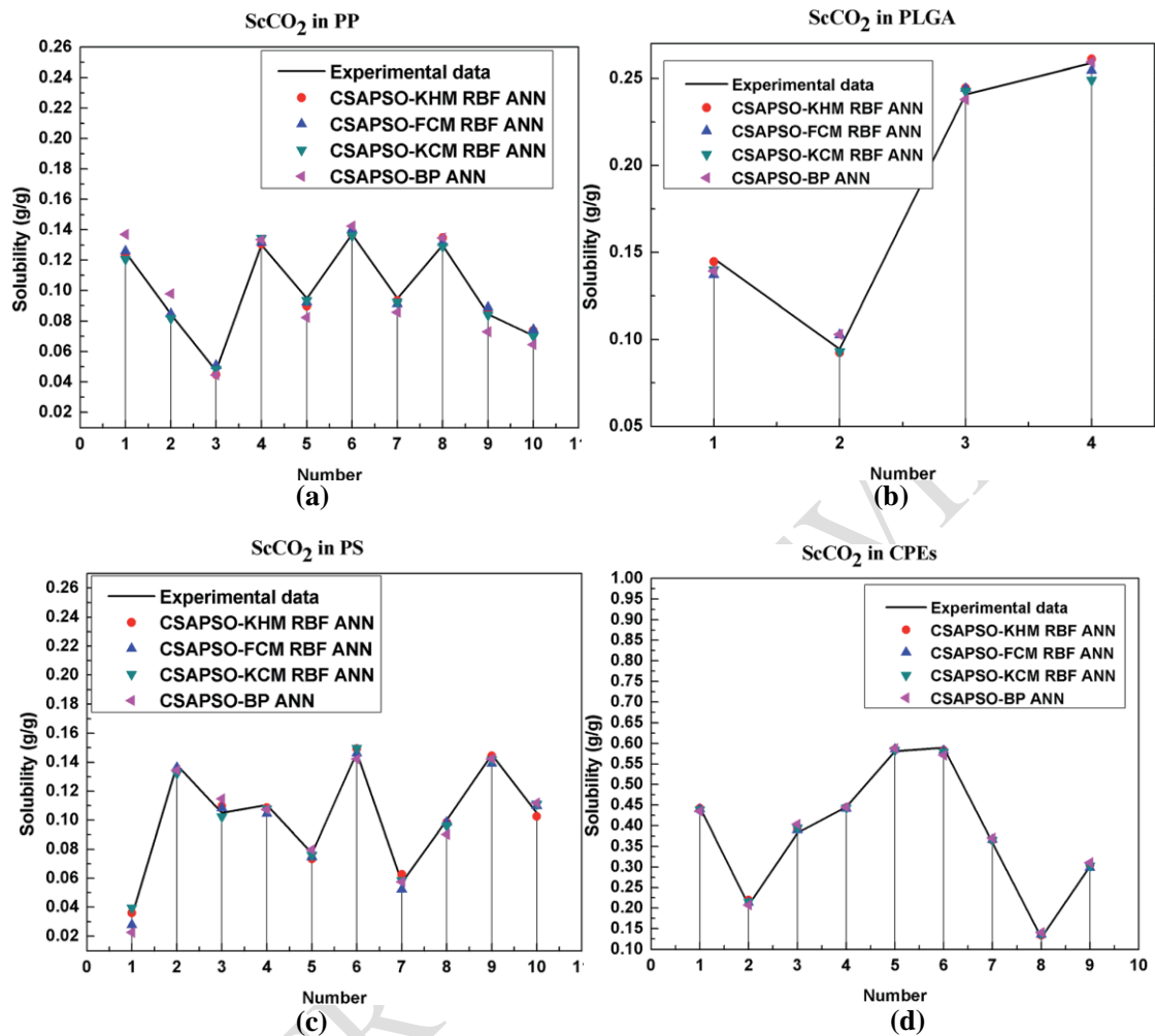
Fig. 7 Prediction of \text{ScCO}_2 in 4 polymers[35]
