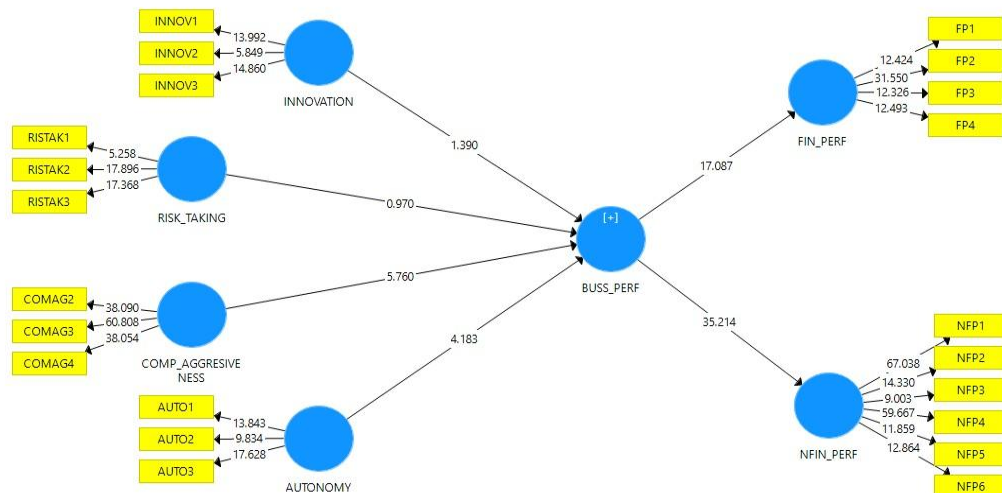
Figure1.PLS-SEM Bootstrapping Model
