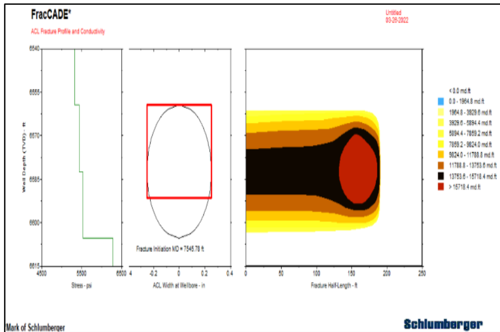
Fig. 2. Fracture geometric
