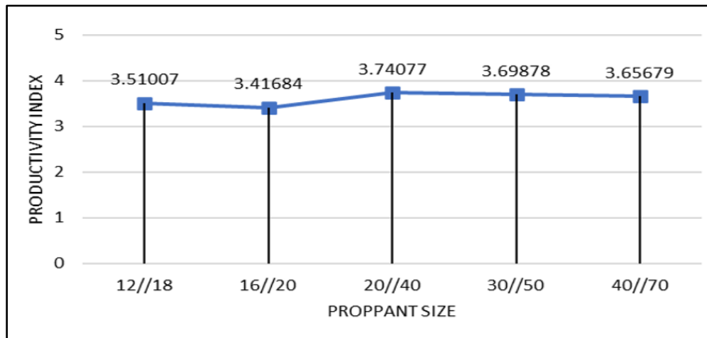
Fig. 4. Productivity index vs proppant size
