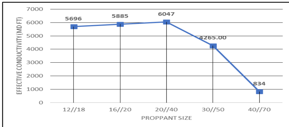
Fig. 3. Fracture conductivity vs proppant size
