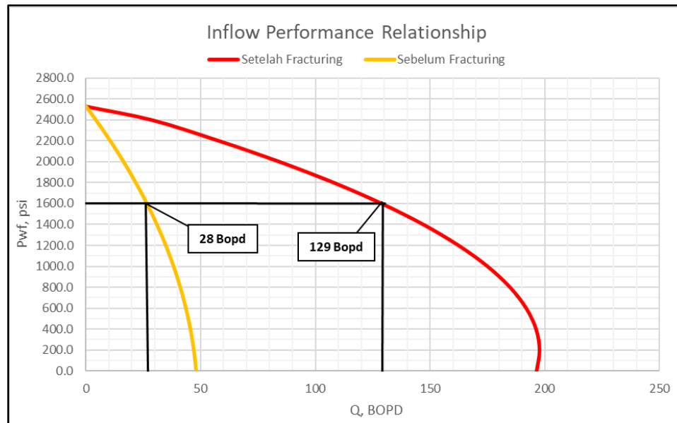
Fig. 5. Comparison of IPR charts before and after hydraulic fracturing
