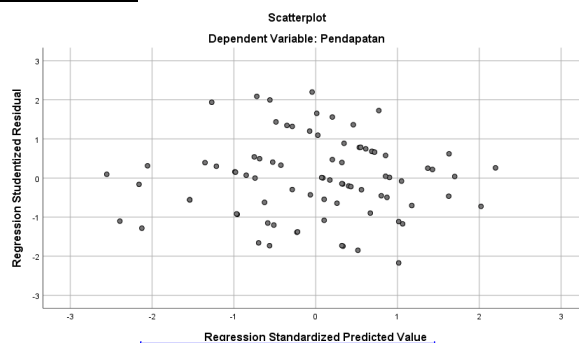
Fig 1. Heteroscedasticity Test
