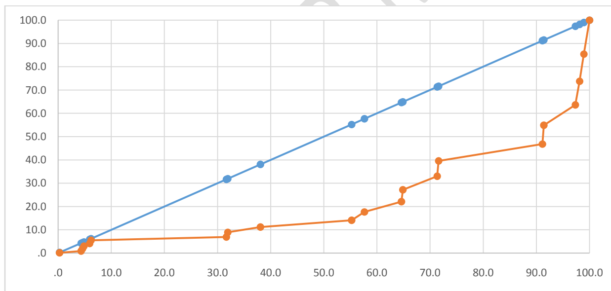
Figure 1 Lorenz Curve of Medical Expenditure
