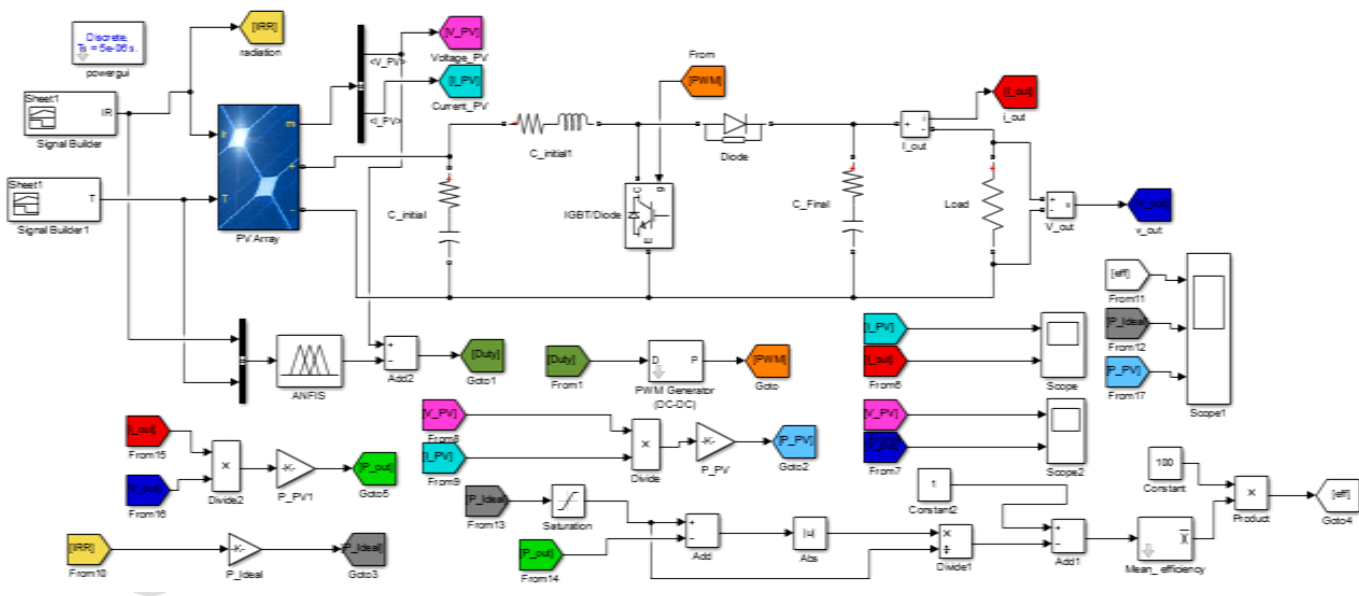
Figure 8: Simulink model for ANFIS based MPPT Charge Controller
