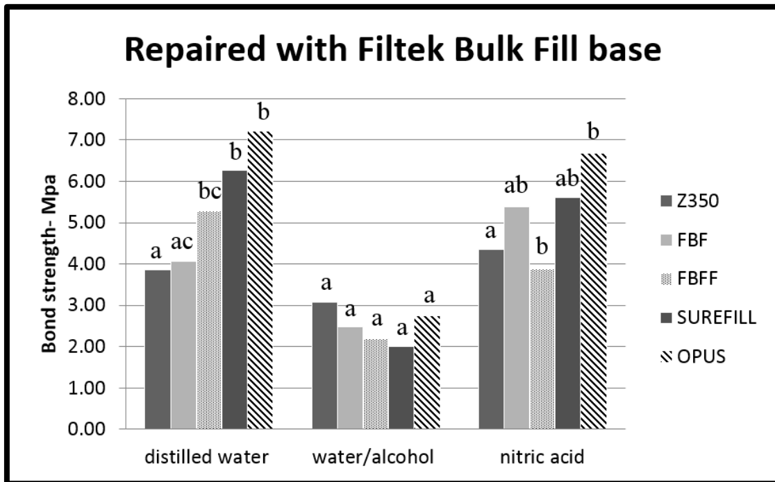
Figure 3 Bond strengths in the tensile tests with the Filtek Bulk base samples in the experimental groups, analysis intrasolution (MPa).
