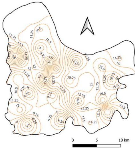
Fig. 6(a). Pre-monsoon depth to water table contour map during the year 2015.
