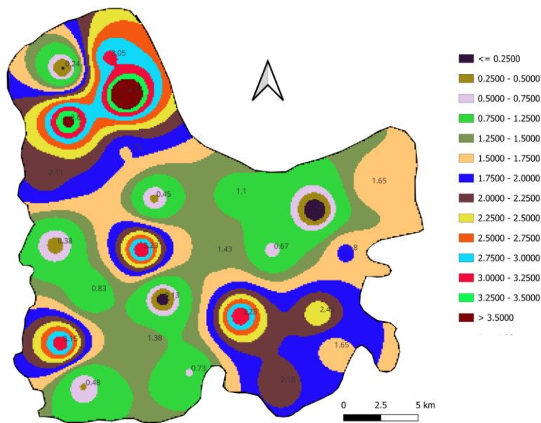
Fig. 8. Average yearly seasonal fluctuation of groundwater table (1997-2003).
