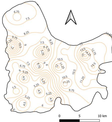
Fig. 3(a). Pre-monsoon water table depth contour map during the year 1997.
