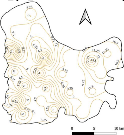
Fig. 5(b). Post-monsoon water table depth contour map during the year 2009.
