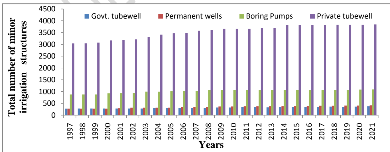
Fig. 13. Variation of total number of minor irrigation structures during year 1997-2021.
