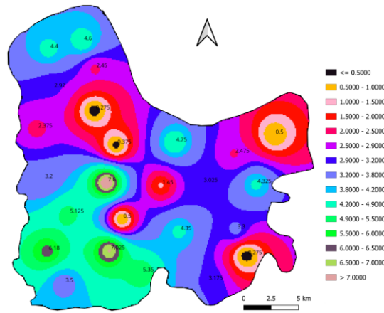
Fig. 12. Average yearly seasonal fluctuation of groundwater table (1997-2021).
