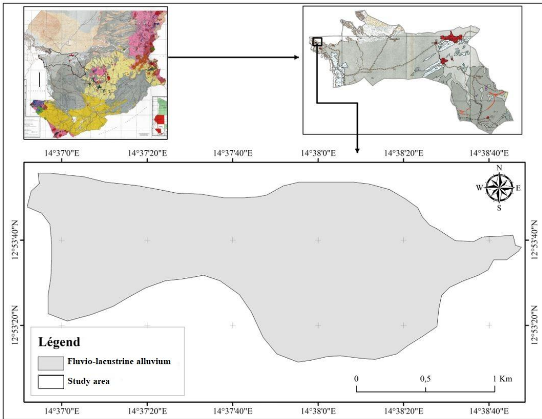
Figure 5 :Geological map of the study area[11]
