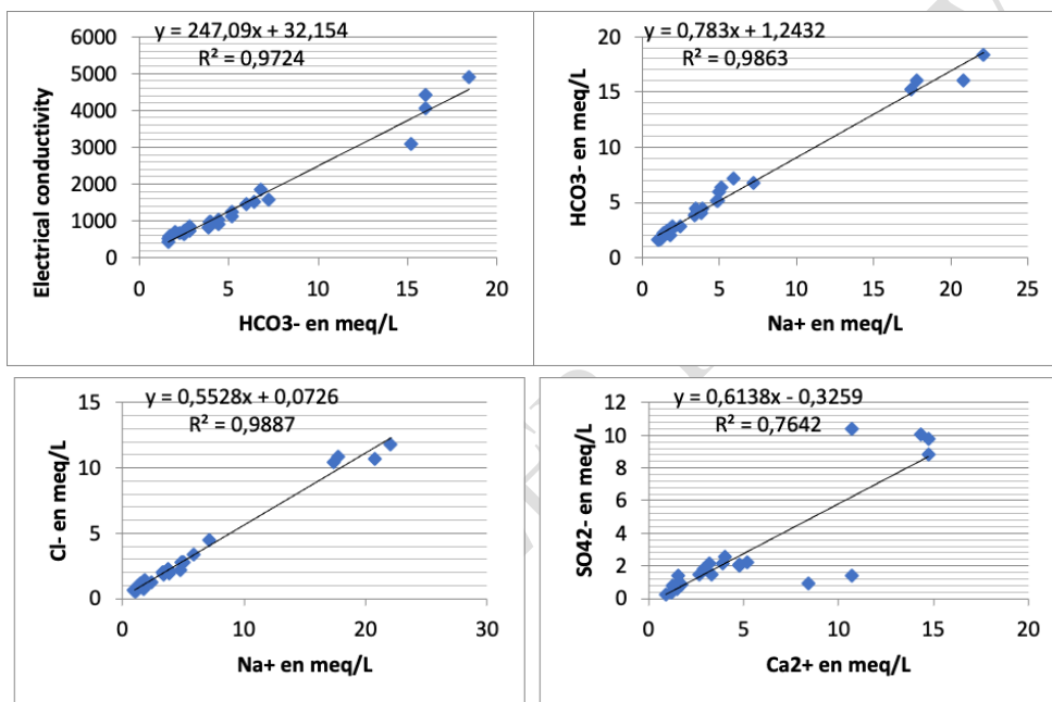
Figure 12. Relationship between chemical elements
