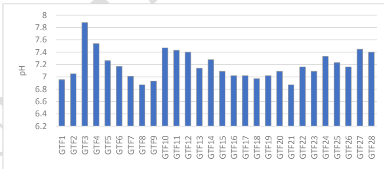
Figure 7. pH in groundwater
