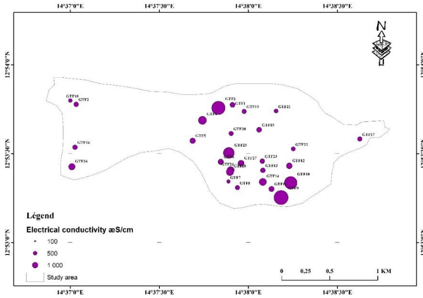
Figure6. Spatial distribution map for electrical conductivity
