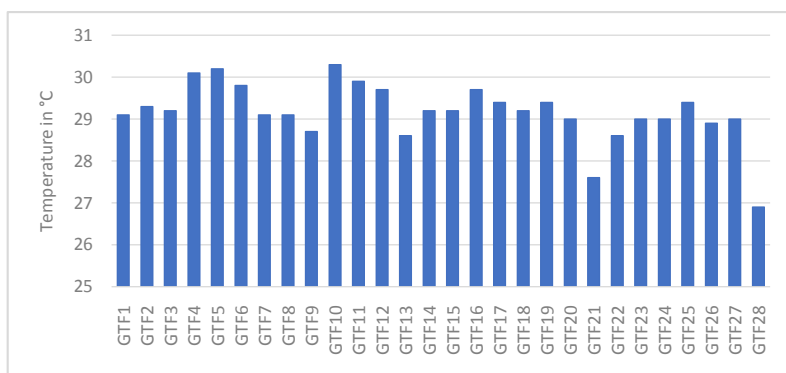
Figure5.Variation in water temperature
