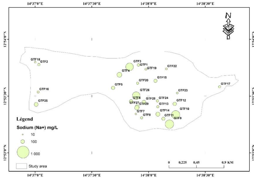
Figure 11. Spatial distribution map of groundwater in sodium
