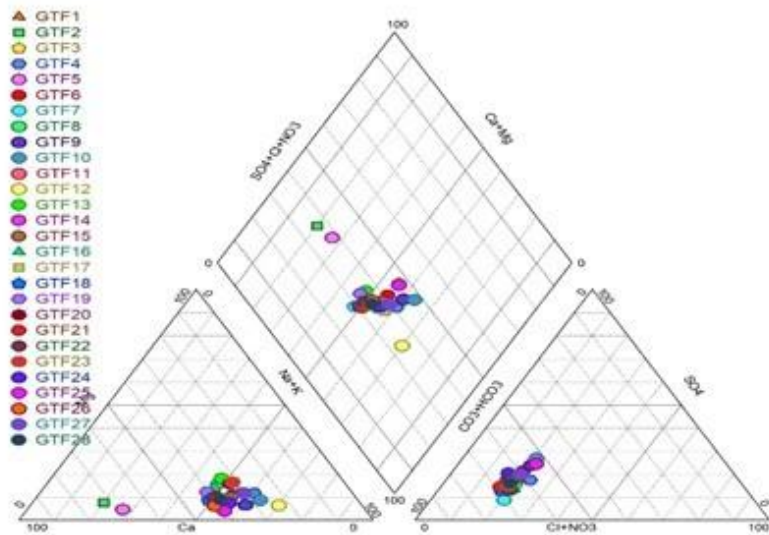
Figure 9. Groundwater hydrochemical facies at Guitté
