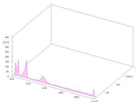
Figure No.2 3D Chromatogram
