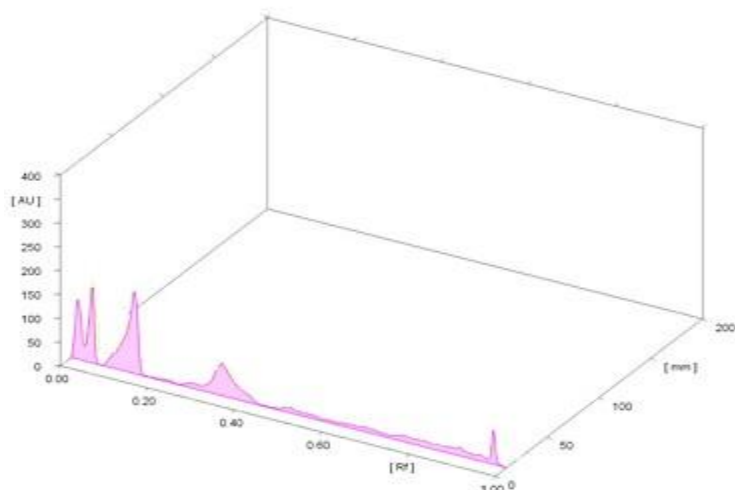
Figure No.2 3D Chromatogram
