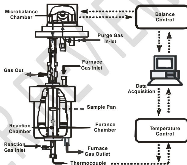
Figure 1: Schematic diagram of the TGA.
