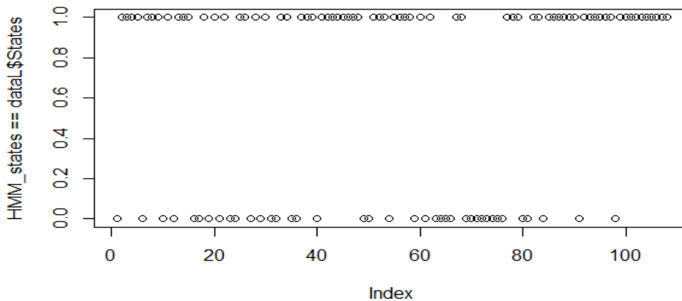
Figure 4: Comparison of Actual Hidden Sequence to Predicted Hidden Sequence
