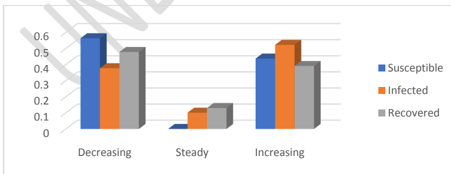
Figure3: Graphical Representation of Emission Probability Matrix
