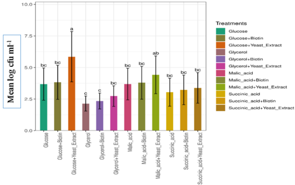
Fig 1. Growth of A. lipoferum Az 204 in media containing different Carbon sources and growth promoting nutrients. (Since the P-value in ANOVA table is < 0.05, there is a significant difference between atleast a pair of treatments) For each carbon source, values denoted with different lower case letter differ significantly at P<0.05 by one-way ANOVA and Tukey's post hoc analyses. The bar represents the significant differences between the treatments.
