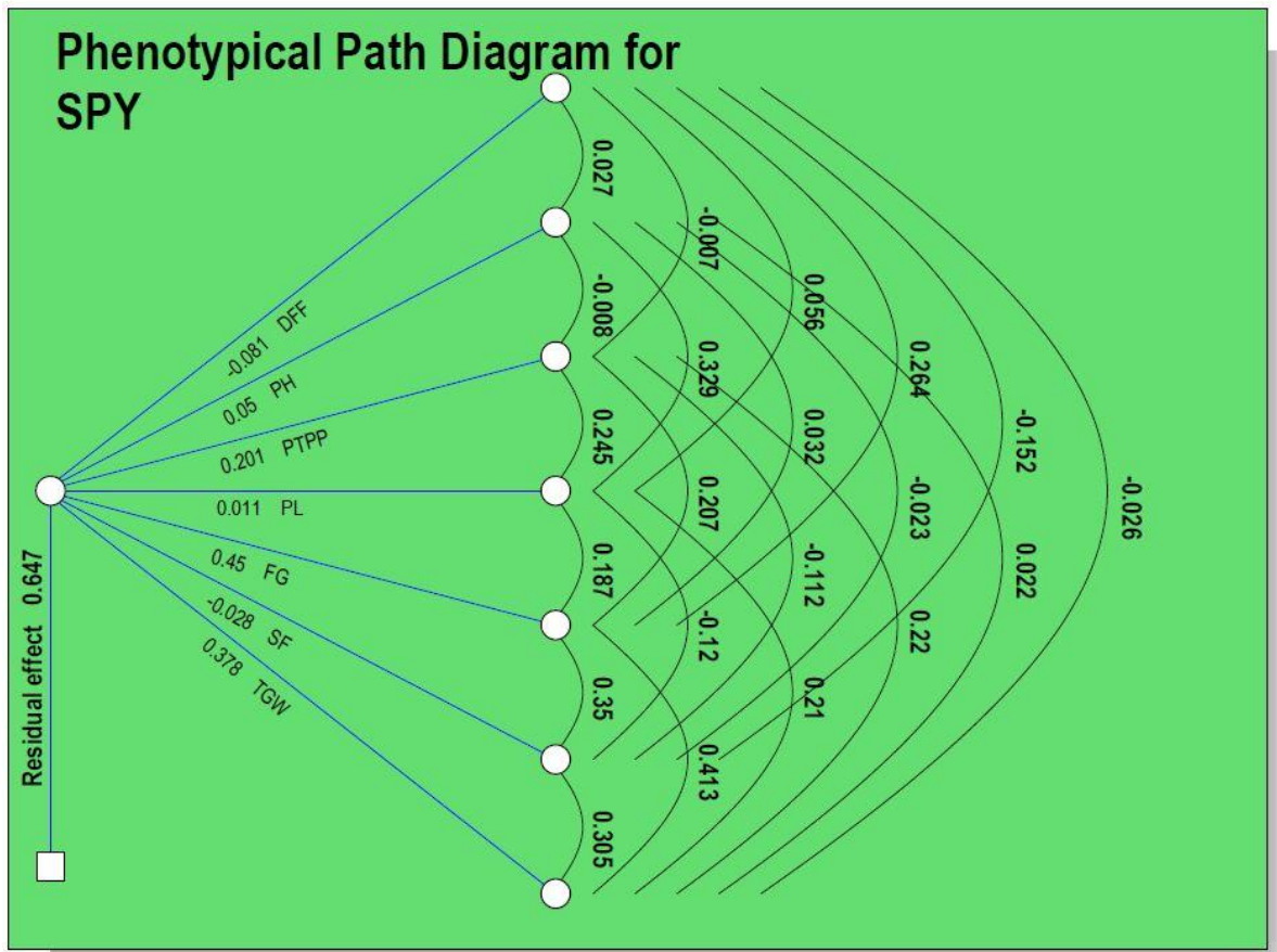
Fig 3: Phenotypic path diagram
