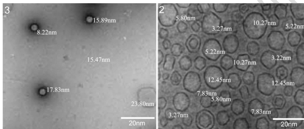
Figure 6: TEM monograph of Calcined kaolin
