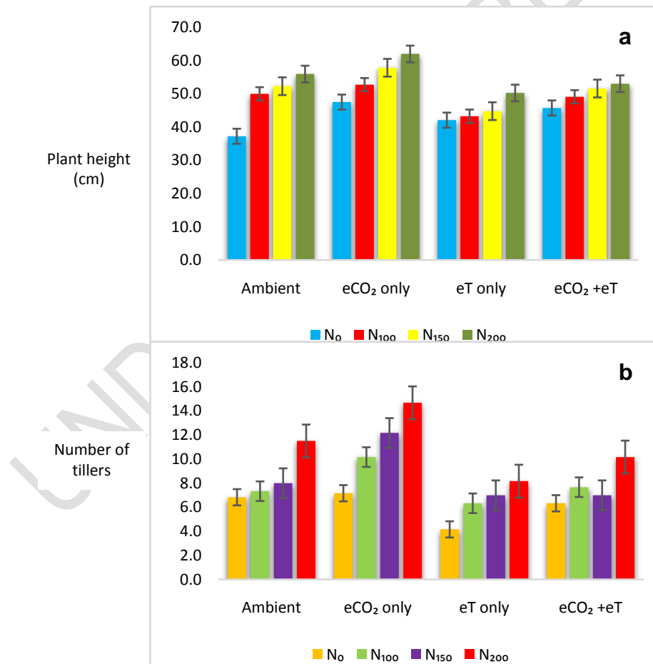
Fig 1. Effect of Open Top Chamber treatments and nitrogen levels on plant height (a) and number of tillers (b) of rice at active tillering
