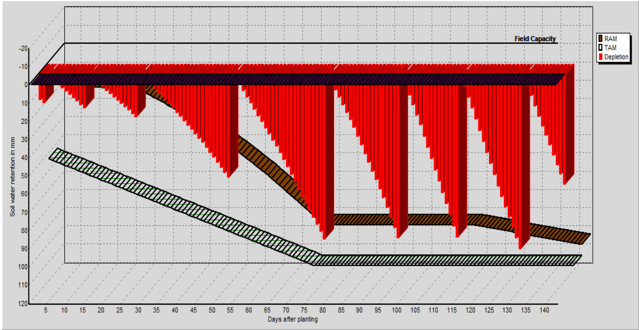
Figure 2: Irrigation scheduling graph for alfalfa crop during crop cycle
