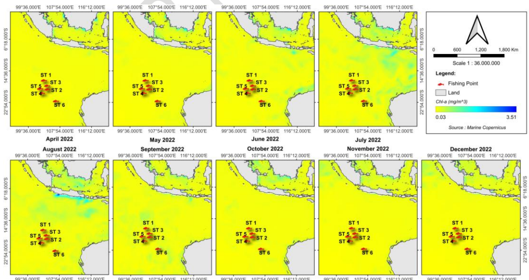
Fig 4. Distribution of Chlorophyll-a from April 2022 to December 2022
