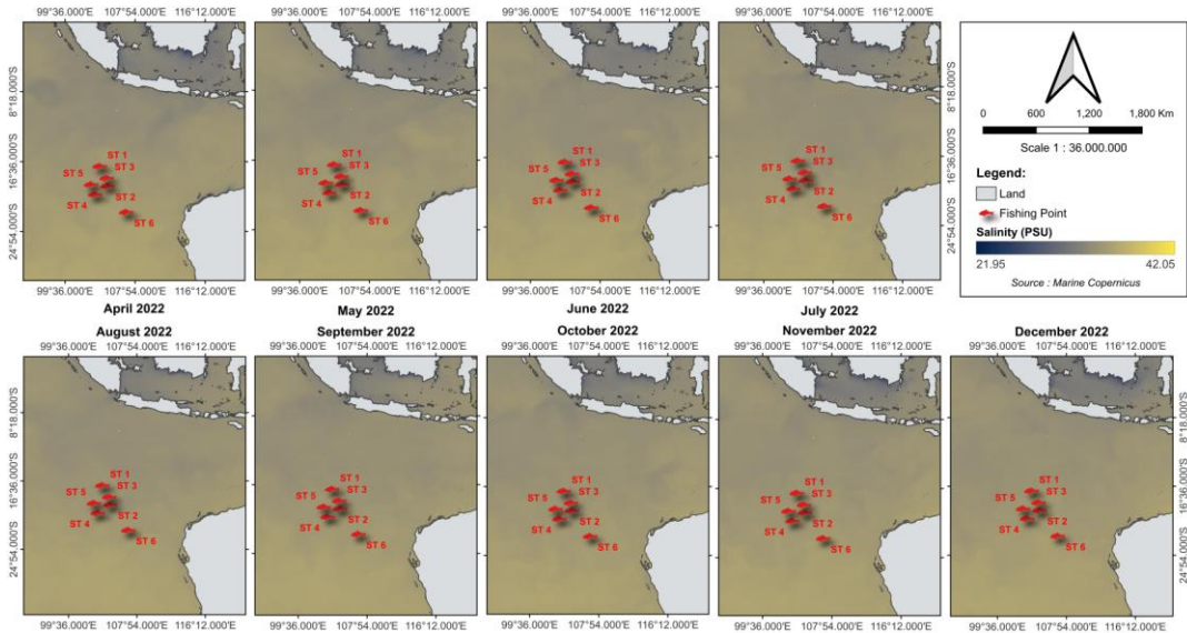
Fig 3. Distribution of Salinity for the Period April 2022 – December 2022.
