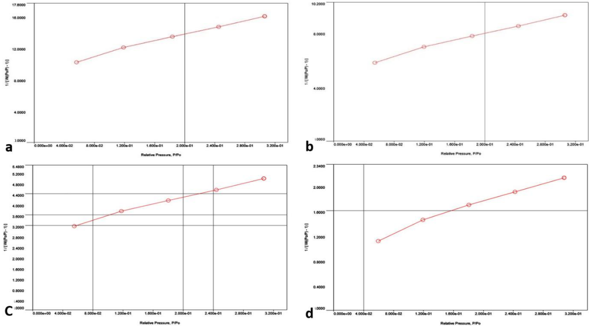
Fig. 3. Nitrogen (N 2 ) Adsorption Isotherm of Carbonized and Chemically Activated Peat Samples. (a) PAC-D: Carbonized; (b) PAC-ZC: Activated with ZnCl 2 ; (c) PAC-HP: Activated with H 3 PO 4 ; (d) PAC-ZC+HP: Activated with ZnCl 2 & H 3 PO 4
