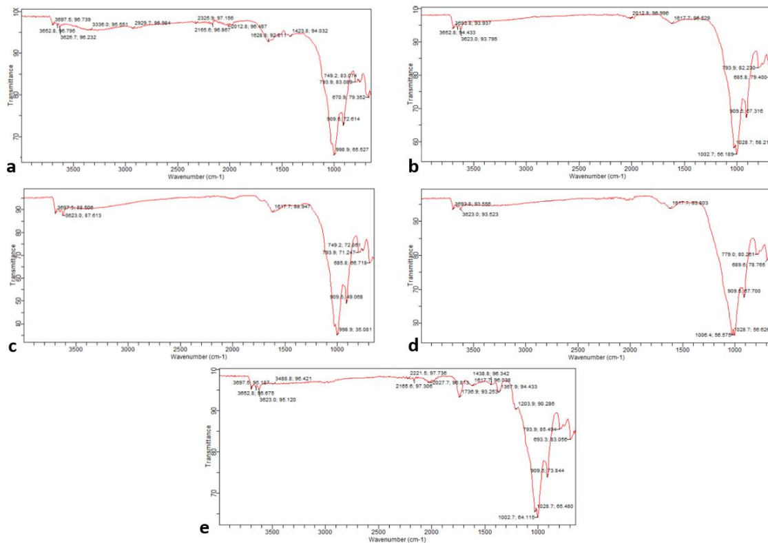
Fig. 1. FTIR Spectra of Raw, Carbonized, and Chemically Activated Peat: (a) RP: Raw Peat; (b) PAC-D: Carbonized; (c) PAC-ZC: Activated with ZnCl 2 ; (d) PAC-HP: Activated with H 3 PO 4 ; (e) PAC-ZC+HP: Activated with ZnCl 2 & H 3 PO
