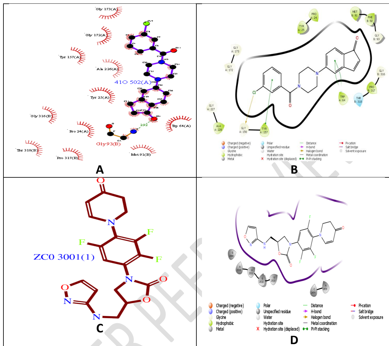
Figure 2. A) Ligplot and B) 2D Complex of Pretomanid with 4XJOC) Ligplot and D) 2D Complex of Contezolid with 6WQN
