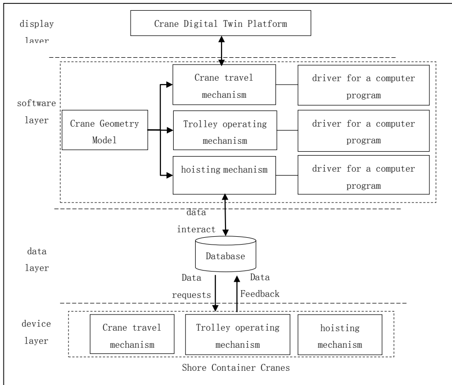
Fig. 4 Port Crane Digital Twin System Architecture
