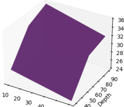
Fig 2C: Total Dissolved Solids y = -0.0679 \times \text{hhr} + 0.1419 \times \text{depth} + 25.0526
