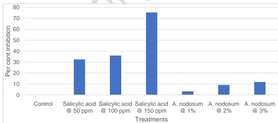
Figure 2. Effect of elicitors on the mycelial growth of Alternaria brassicae
