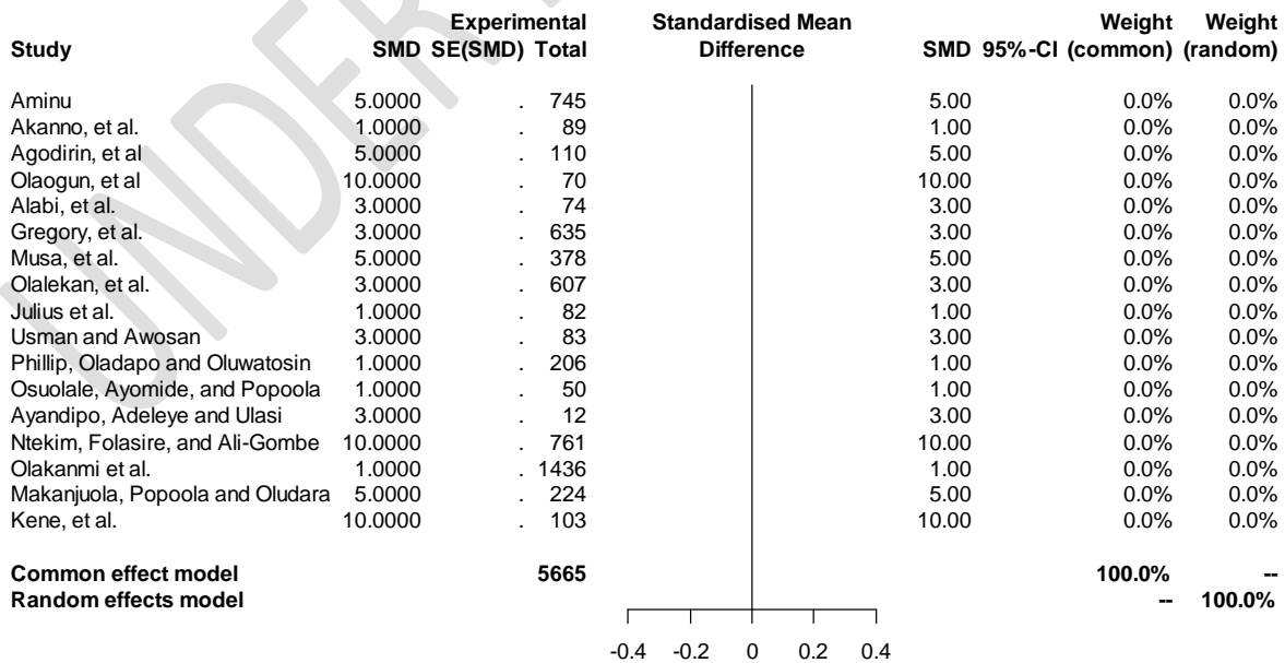
Chart 1: Forest plots
