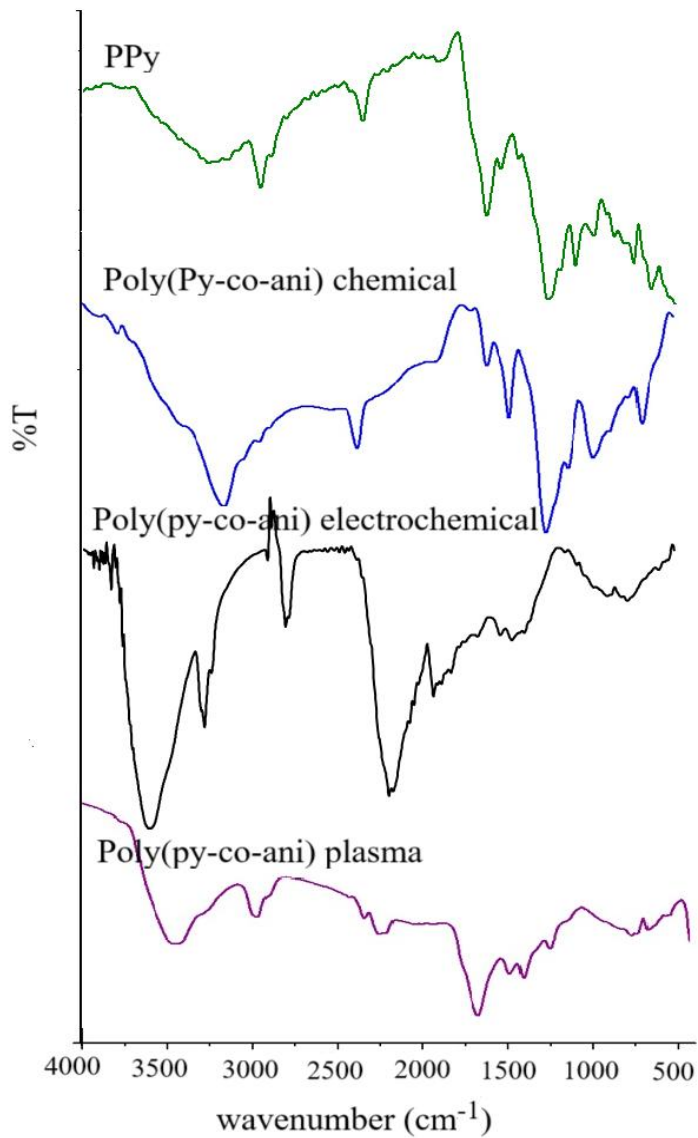
Figure 1. FTIR spectrum of Ppy and copolymers
