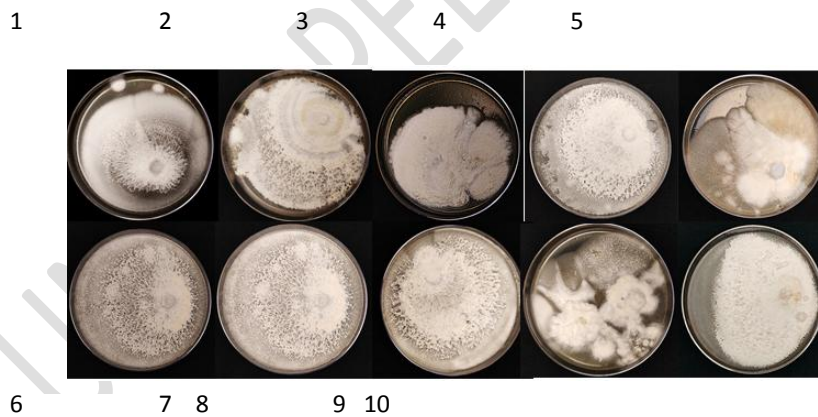
Figure.2 Isolation of U. virens in PSA medium
