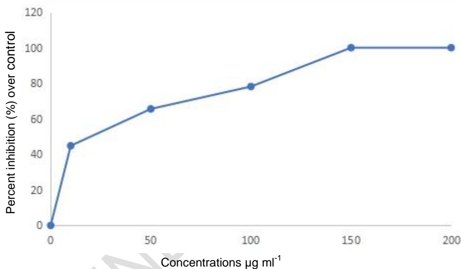
(b) Dose response curve of M. phaseolina to carbendazim on agar plate.
