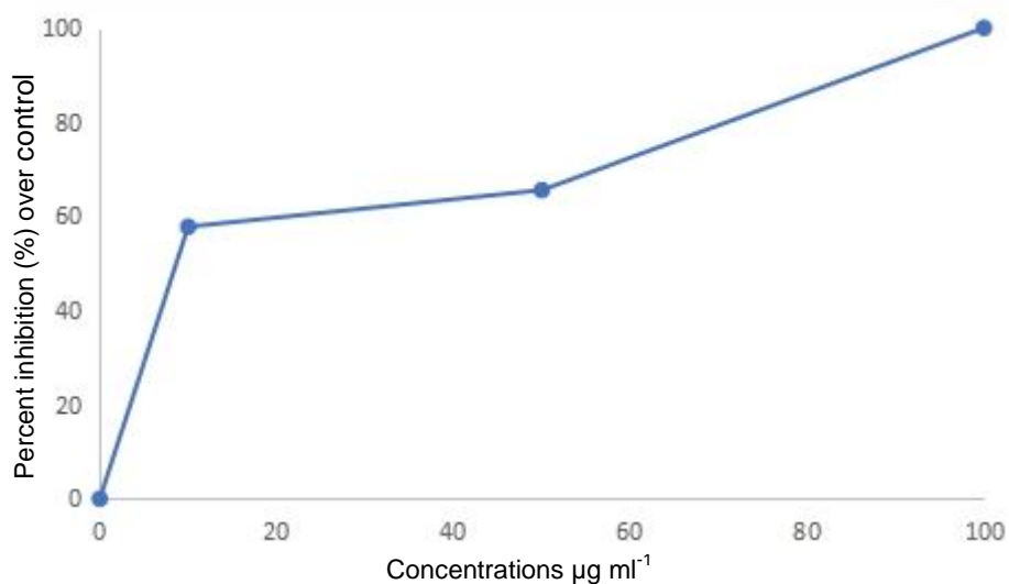
(b) Dose response curve of F.oxysporum to carbendazim on agar plate.
