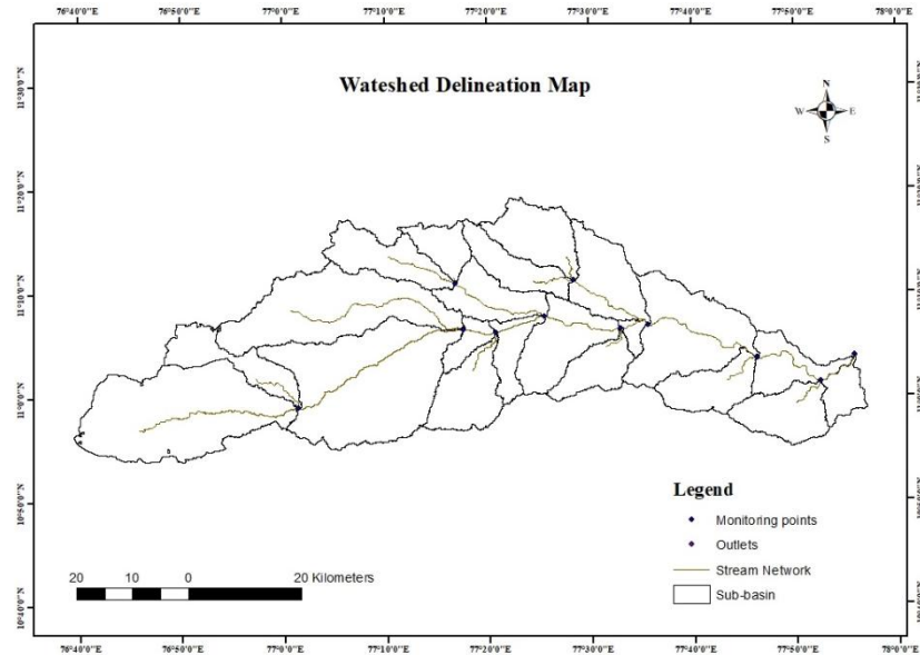
Fig.4. Delineation of Sub-basin of Noyyal River Basin
