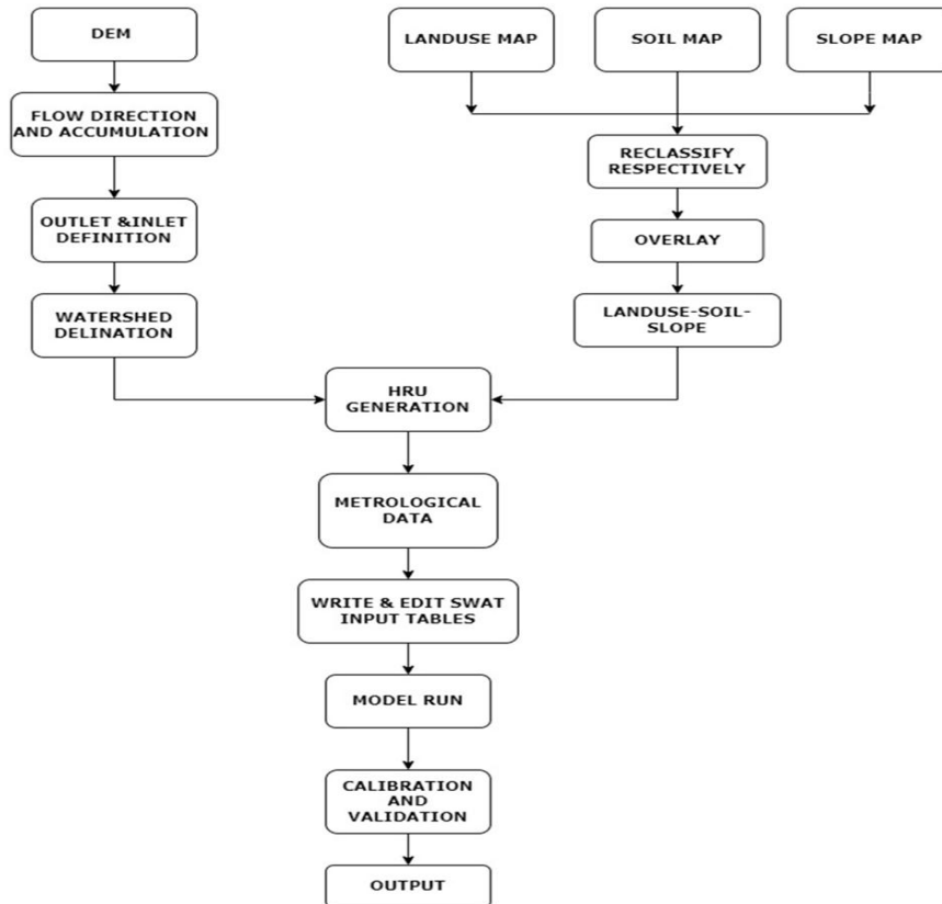
Fig.2. Flowchart for Runoff assessment using SWAT
